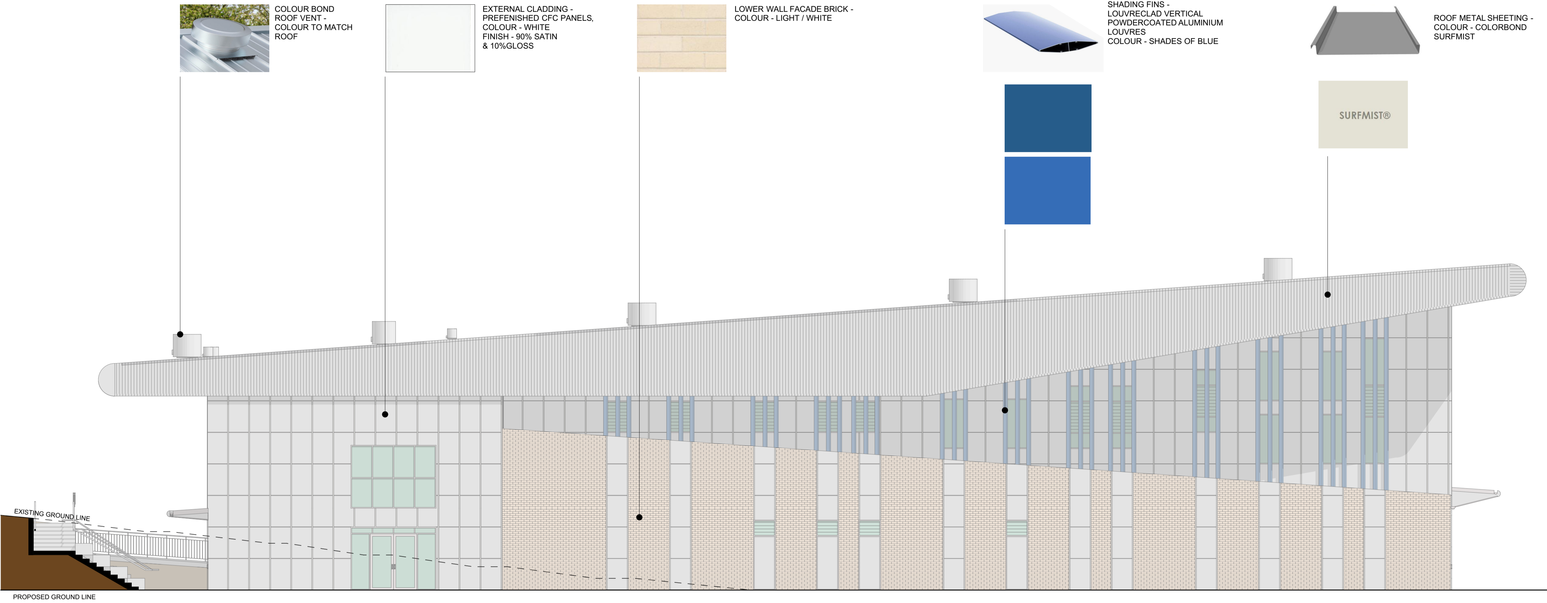
1 WEST ELEVATION - COLOURS & MATERIALS 1:100
